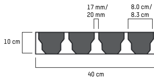
Sows slatted floor in profile
