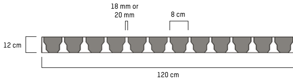
Pig slatted floor in profile
